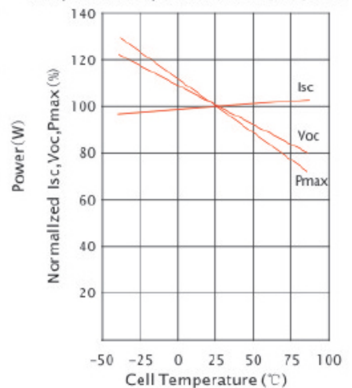
Temperature Dependence of Isc, Voc, Pmax
