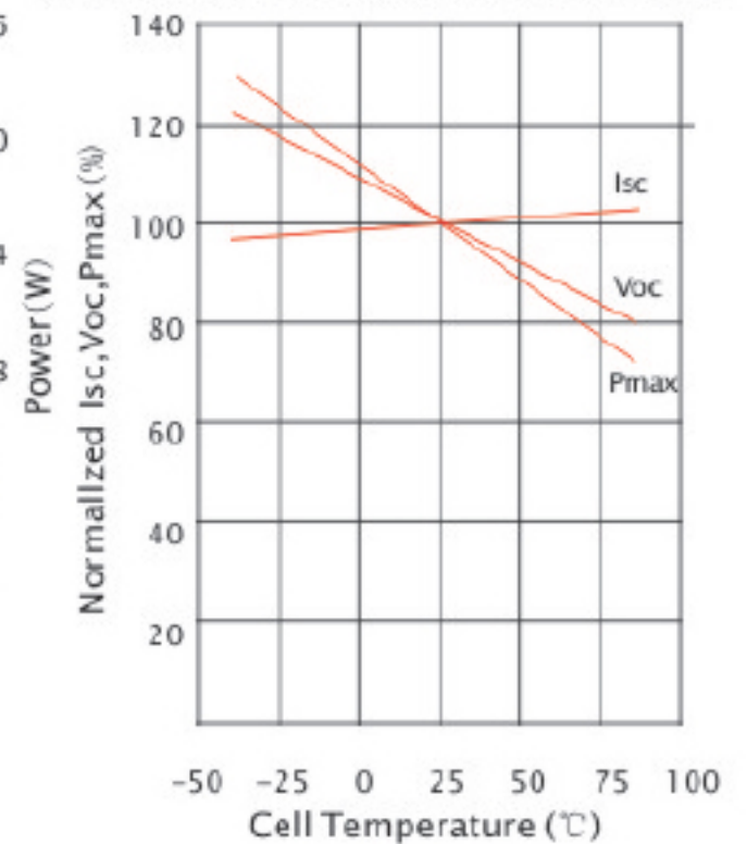
Temperature Dependence of Isc, Voc, Pmax
