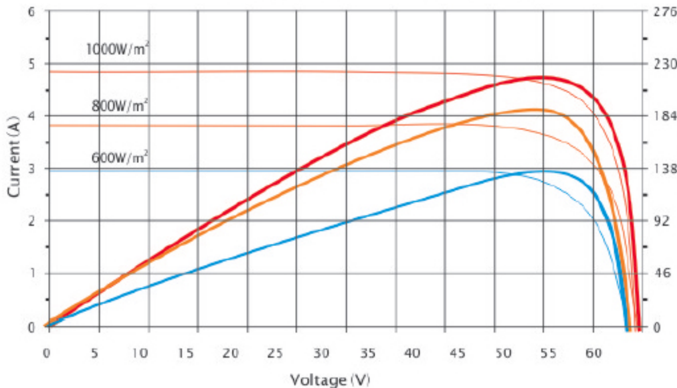
Current-Voltage&Power-Voltage Curve (220W)
