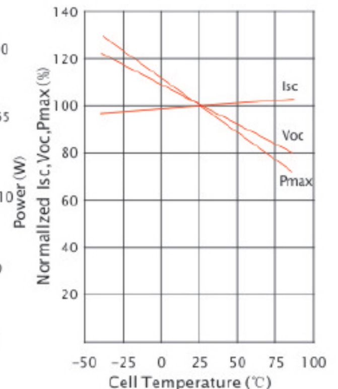
Temperature Dependence of Isc, Voc, Pmax
