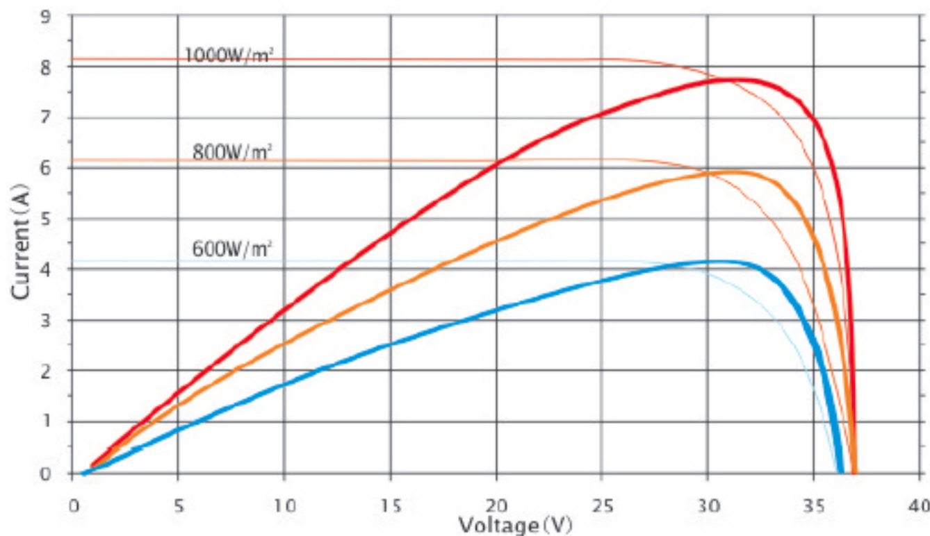
Current-Voltage&Power-Voltage Curve(220W)
